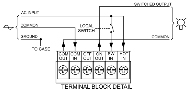
Diagram 4. SWITCHED LOADS
